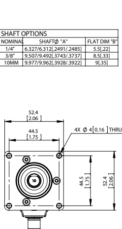
SQUARE FLANGE
